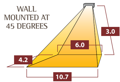
Coverage area = 35.3m sq.
