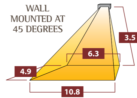
Coverage area = 41.6m sq.
