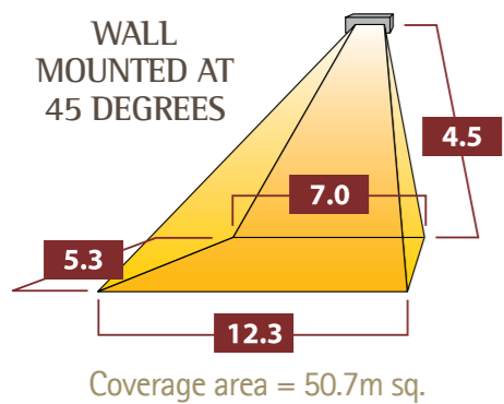
Apollo mounted at 4.5m from floor
