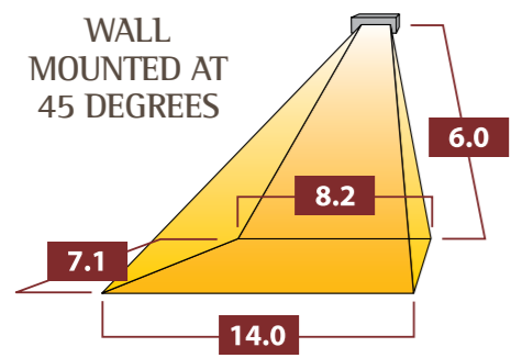
Coverage area = 79.0m sq.
